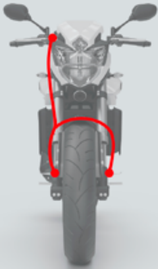
3 LINE FRONT WITH T-PIECE
